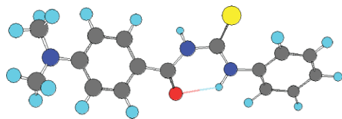
Scheme 2 AM1 optimized structure of 1b .
